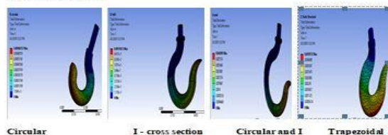
Deformation of hook
