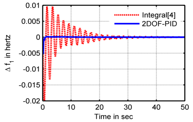
Fig. 4: Frequency Oscillations in Area 1.
