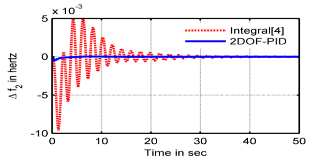
Fig. 5: Frequency Oscillations in Area 2.
