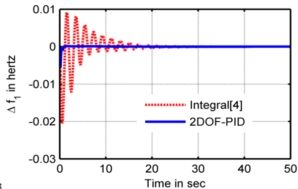
Fig. 8: Frequency Oscillations in Area 1 with Delay.
