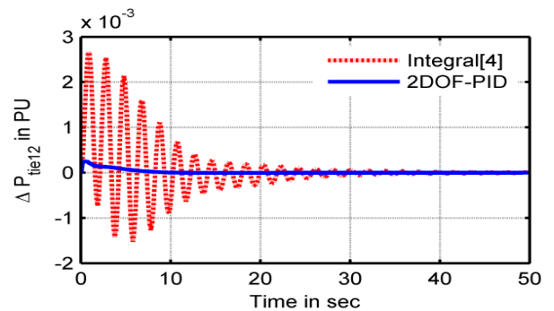
Fig. 7: Tie-Line Power Oscillations between Area 1&2.
