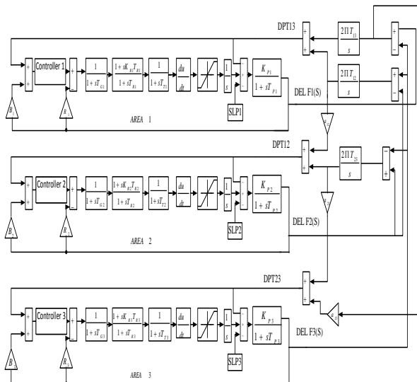
Fig. 1: Three Area Unified System with GRC.
