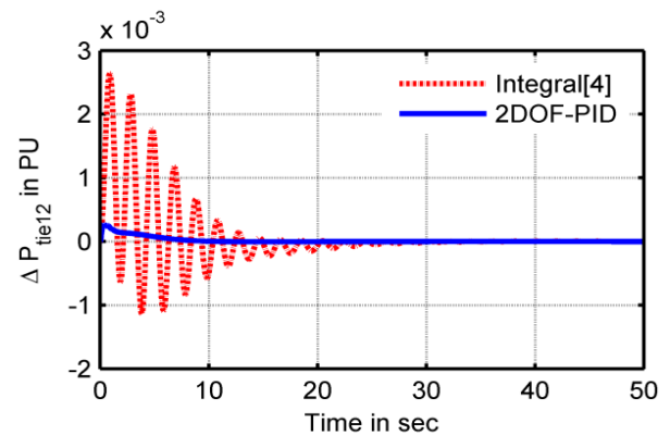
Fig. 9: Tie-Line Power Oscillations with Delay
