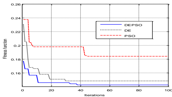
Fig. 3: Convergence Behavior of Different Optimization Methods.
