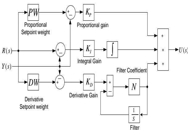
Fig. 2: Outline of 2-DOF PID Controller.
