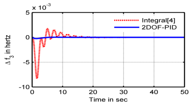
Fig. 6: Frequency Oscillations in Area 3.
