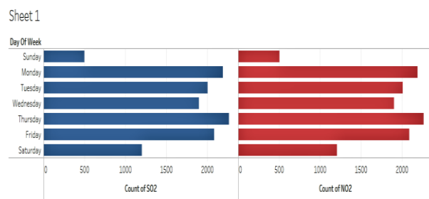
Fig. 5: Tamilnadu Data Based on Pollutants and Weekdays.
