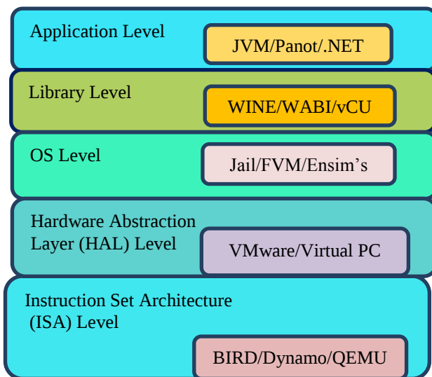
Fig. 2: Implementation Levels of Virtualization.
