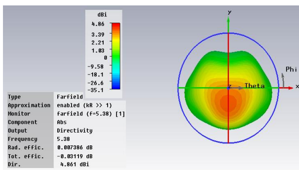
Fig. 4: 3-D Radiation Pattern Showing Directivity of Proposed Receiver Antenna.
