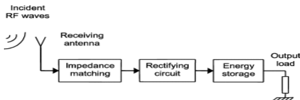
Fig. 1: General Diagram of Rectenna Circuit.
