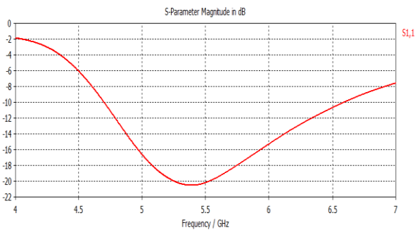
Fig. 3: Return Loss vs Frequency Plot of Proposed Antenna.
