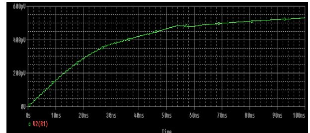
Fig. 7: Output Voltage across Load R1 (Mv).
