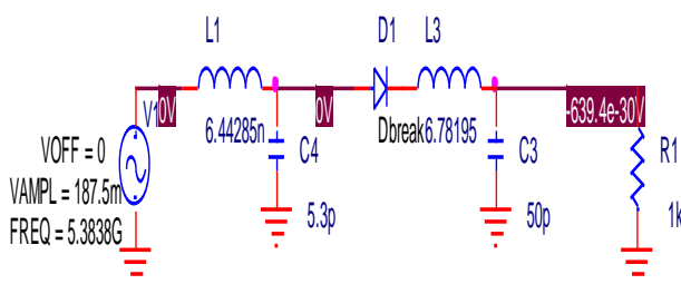
Fig. 5: Rectifying Circuit.
