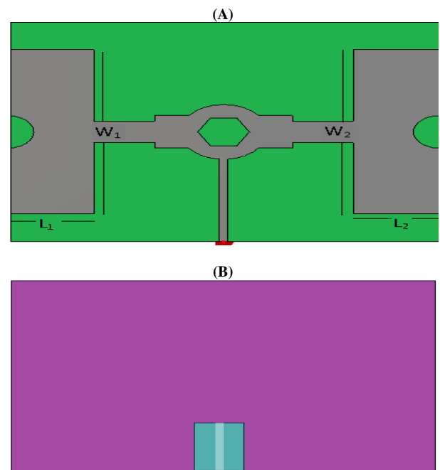
Fig. 2: Proposed Antenna Partial Ground Plane.
