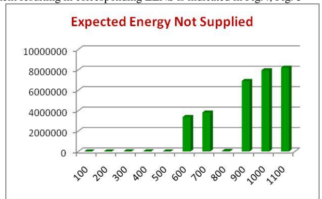
Fig. 3. Expected energy not supplied for load at bus three
