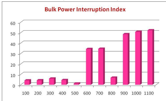
Fig. 5. Overall system bulk power interruption index Vs load variation
