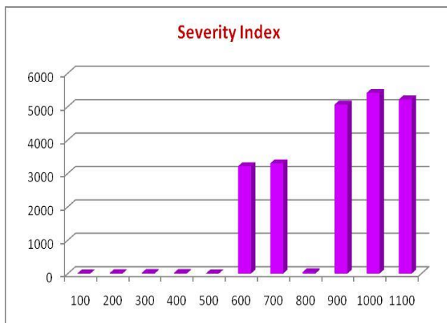
Fig. 6. Overall system Severity index Vs load variation
