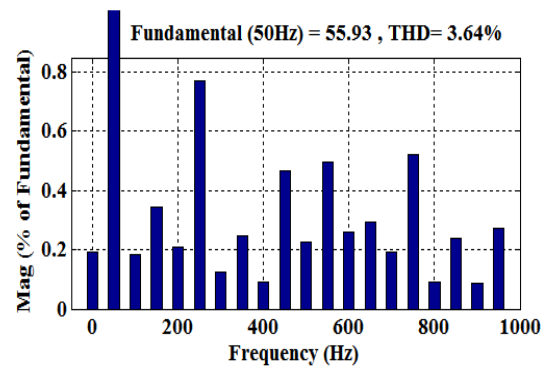
Fig.7(a): Current THD at PCC (BUS-2)
