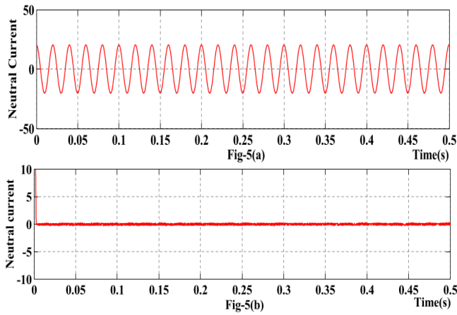
Fig-5. (a). Neutral current wave form without compensation, (b). Neutral current wave form after compensation.
