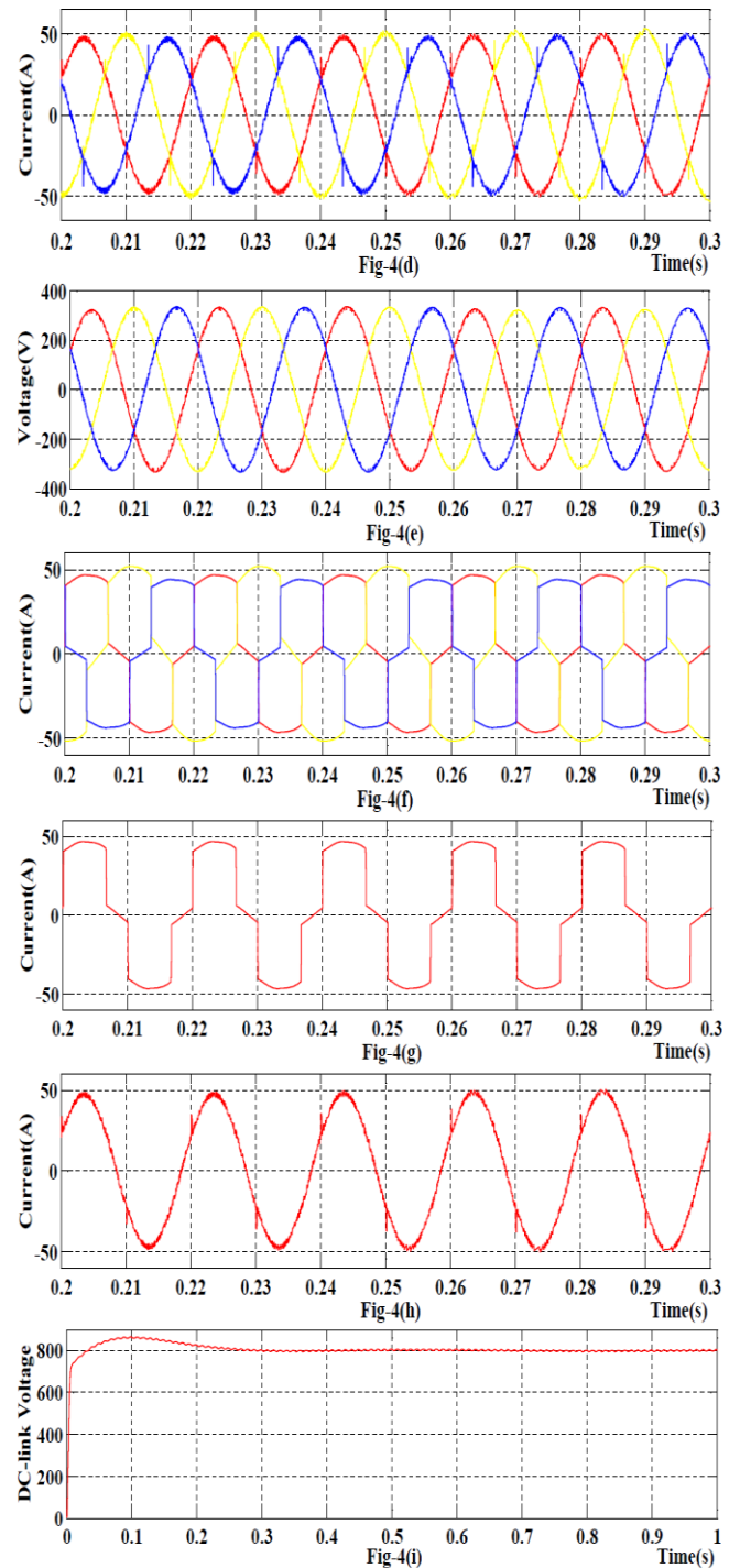
Fig. 4: (a) Source voltage wave form, (b). Source current wave form, (c).voltage waveform at the PCC (Bus-2), (d). Current waveform at the PCC (Bus-2), (e).Load voltage wave form, (f).Load current wave form, (g). Per phase representation of load current wave form, (h). Per phase representation of current wave form at the PCC (i).DC-link voltage form ( V_{dc} ), with PI controlled D-STATCOM.
