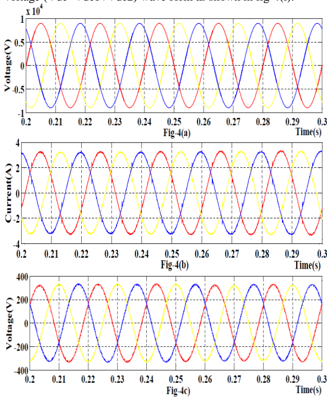
Fig. 4: (a) Source voltage wave form, (b). Source current wave form, (c).voltage waveform at the PCC (Bus-2), (d). Current waveform at the PCC (Bus-2), (e).Load voltage wave form, (f).Load current wave form, (g). Per phase representation of load current wave form, (h). Per phase representation of current wave form at the PCC (i).DC-link voltage form ( V_{dc} ), with PI controlled D-STATCOM.
