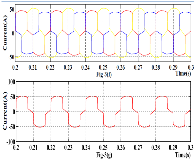
Fig. 3: (a)Source voltage wave form, (b). Source current wave form, (c).voltage waveform at the PCC (Bus-2), (d). Current waveform at the PCC (Bus-2), (e).Load voltage wave form, (f).Load current wave form, (g). Per phase representation of current wave form at the PCC, during unbalanced nonlinear load without D-STATCOM.
