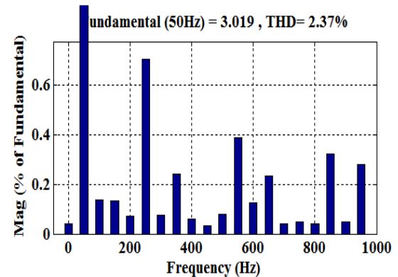
Fig.7(b): Source current THD (BUS-1).
