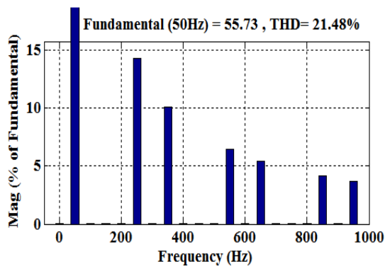
Fig. 6(a): Current THD at PCC (BUS-2)
