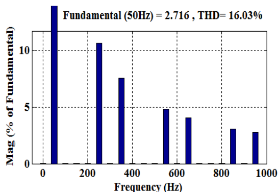
Fig.6 (b): Source current THD (BUS-1)
