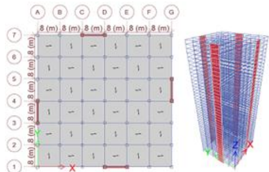
Fig. 2: Plan and 3D geometry of the second model
