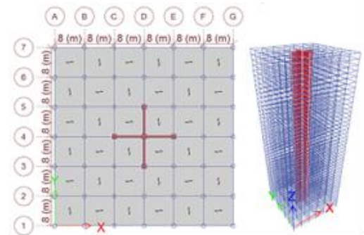
Fig. 6: Plan and 3D geometry of the sixth model
