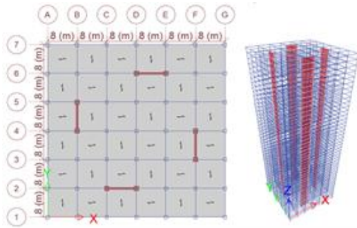
Fig. 3: Plan and 3D geometry of the third model
