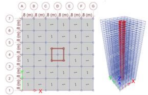
Fig. 5: Plan and 3D geometry of the fifth model
