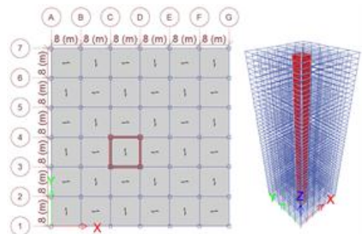
Fig. 7: Plan and 3D geometry of the seventh model
