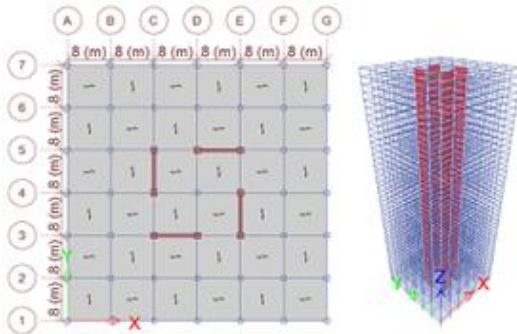
Fig. 4: Plan and 3D geometry of the fourth model
