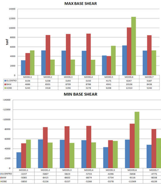
Charts 1: Show comparison of base shear force under different earthquakes in seven geometric models
