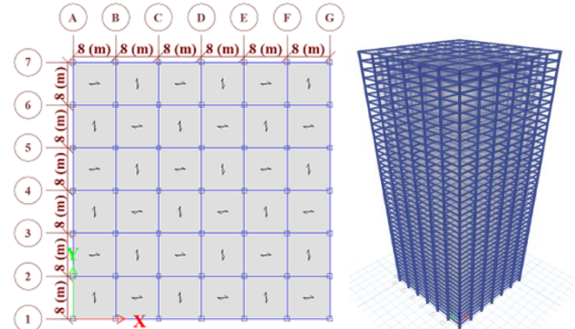
Fig. 1: Plan and 3D geometry of the first model
