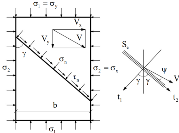
Fig. 1: Kinematically possible failure scheme of concrete plate with biaxial stress state:
