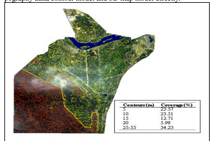
Fig. 2: Contours generated for initial understanding of topography of Pekan sub-district and comparison with 3D generated map model
