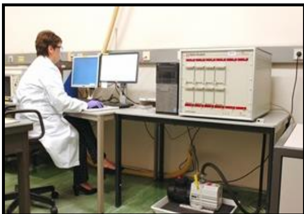
Fig. 5: Alpha Spectrometry
