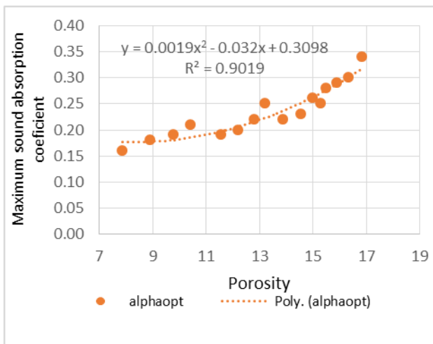
Fig. 9: Relationship between maximum sound absorption coefficient and porosity
