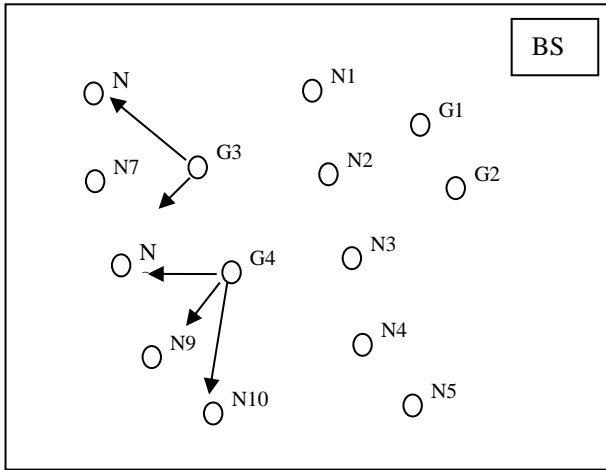
Fig. 2: C) Gateways Transmit Hello Packet.
