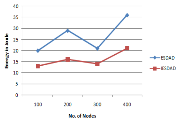
Fig. 5: Energy Consumption Comparison.
