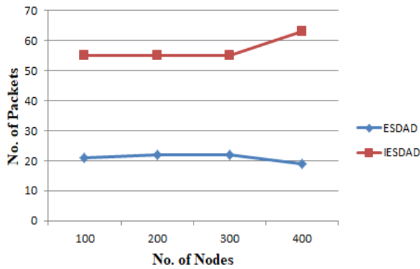
Fig. 6: Throughput Comparison.
