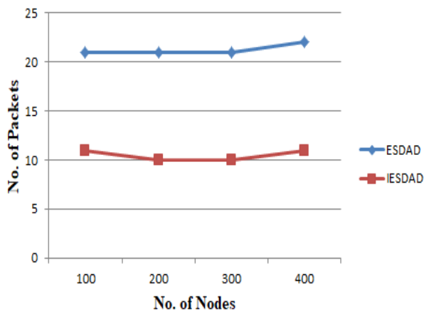
Fig. 8: Packet Loss Comparison.
