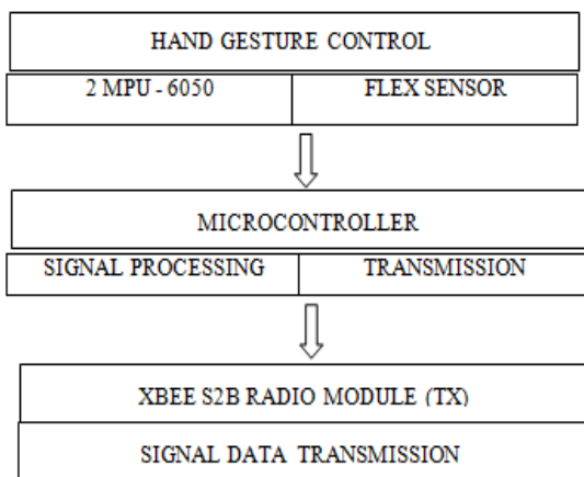
Fig. 3: Signal flow in hand control board
