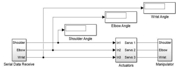
Fig. 5: Simulink model
