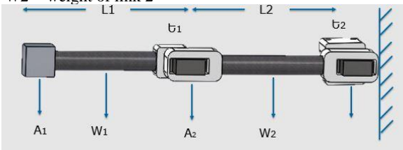
Fig. 8: Manipulator
