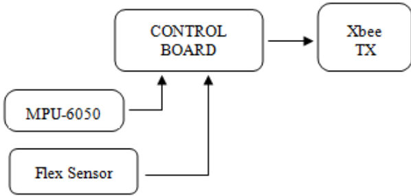
Fig. 1: Block diagram of transmission system
