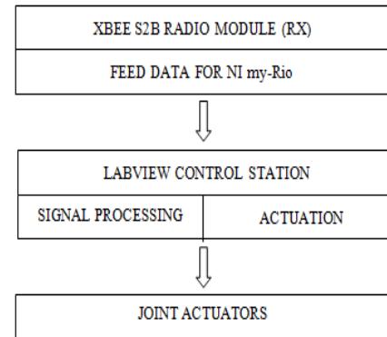
Fig. 4: Signal flow in manipulator control board
