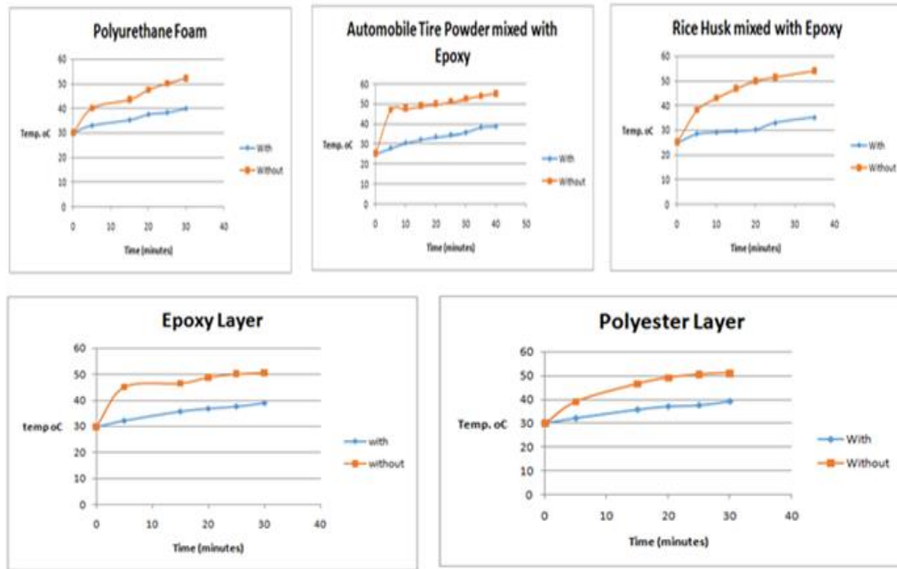
Fig. 6: Temperature Difference Graphs.
