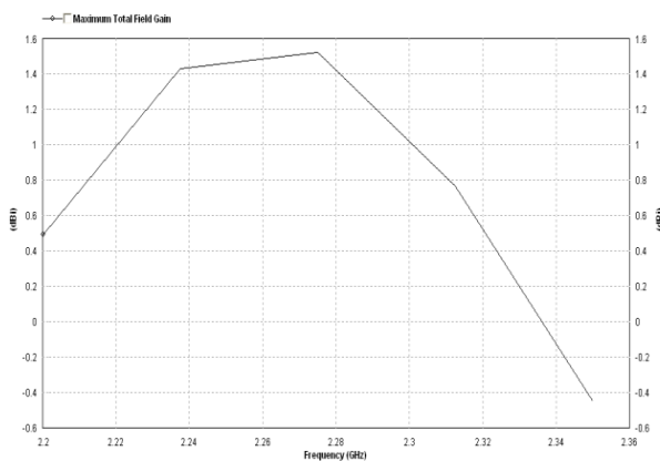
Fig. 6: Total Field Gain vs. Frequency. This Display Gives the Gain Value for the Total Electric Field.
