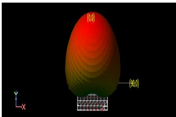
Fig. 2: Three Dimensional Radiation Pattern Display of Rectangular Microstrip Antenna. The red Colour Indicates the Maximum Radiation of Power.
