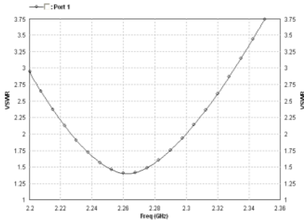
Fig. 5: VSWR Display of Rectangular Microstrip Antenna. For Resonant Bands, It Is Less Than 2.
