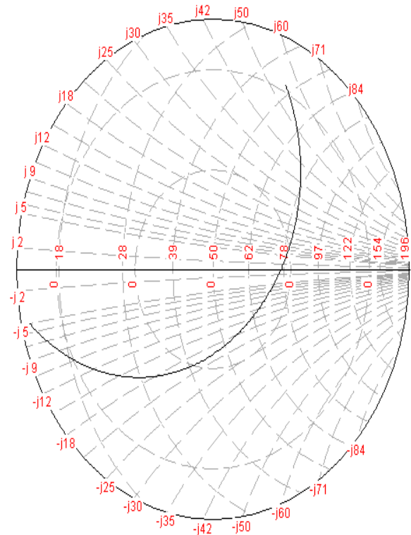
Fig. 3: Impedance Characteristics Display of Rectangular Microstrip Antenna. The Point at Which the Curve and Horizontal Line meets is the Impedance for the Resonant Frequency.
