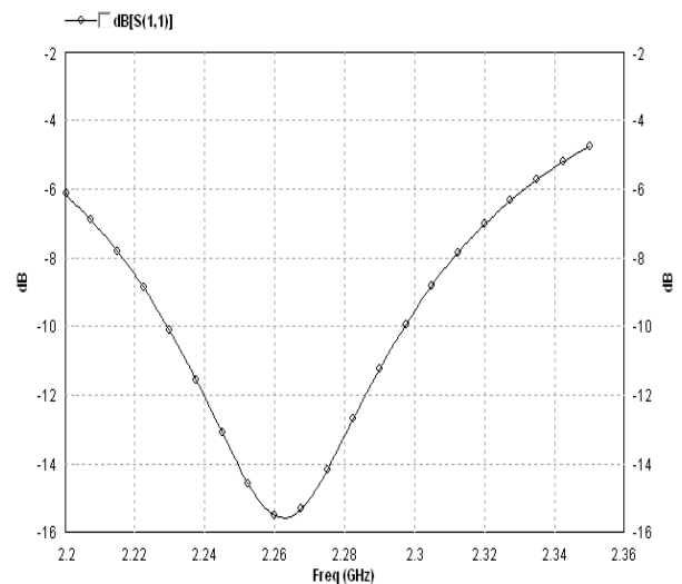
Fig. 4: S-Parameters Display of Rectangular Microstrip Antenna. For the Resonant Band, It Is Less Than -10 dB.
