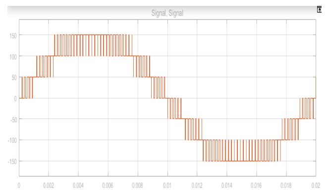
Fig. 8: The output voltage waveform of the CHB-MLI at unity modulation using SPWM-POD technique
