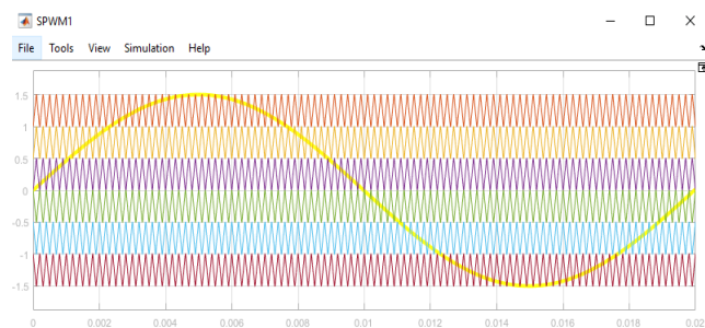
Fig. 5: The modulation signal of a SPWM-PD at unity modulation of the CHB-MLI
