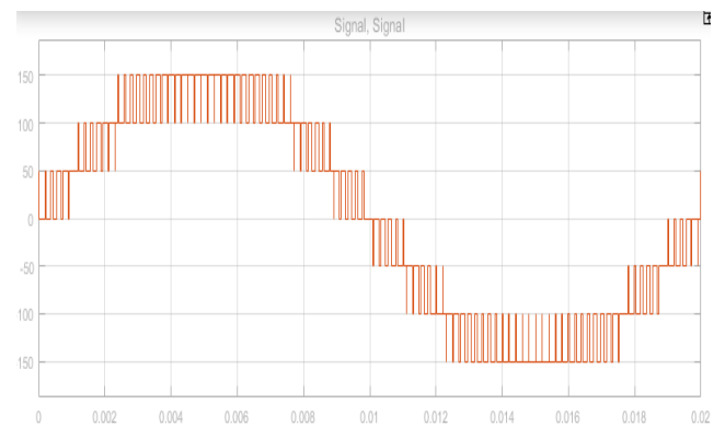
Fig. 6: The output voltage waveform of the CHB-MLI at unity modulation using SPWM-PD technique
