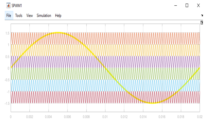
Fig. 7: The modulation signal of a SPWM-POD at unity modulation of the CHB-MLI
