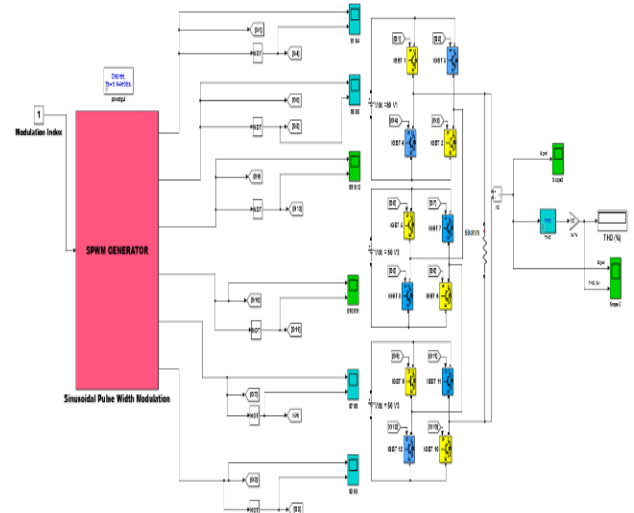
Fig. 2: The single phase 7-level CHB-MLI model
