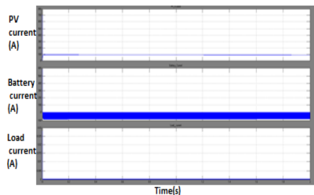
Fig. 7: Current through PV Panel, Battery and Load at Load off Condition.
