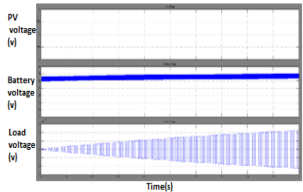
Fig. 6: Voltages of PV Panel, Battery and Load at Load off Condition.
