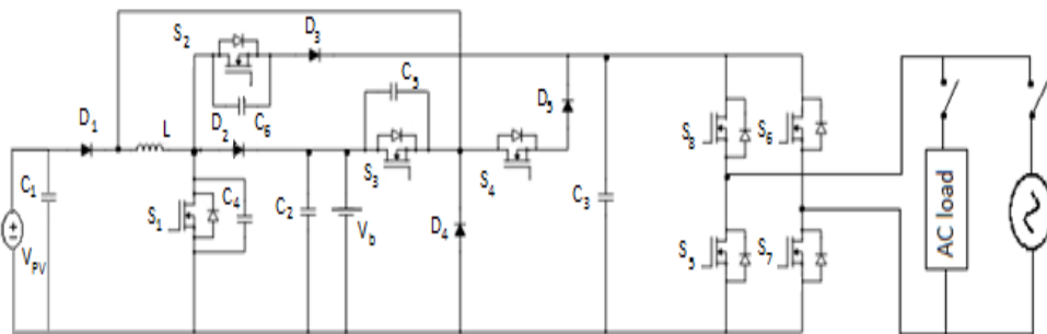
Fig. 1: Proposed Converter Topology.
