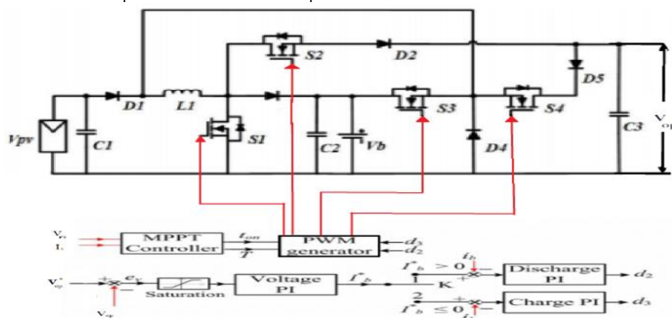
Fig. 3: Three Port Converter with Controller Modeled Using MPPT Algorithm.
