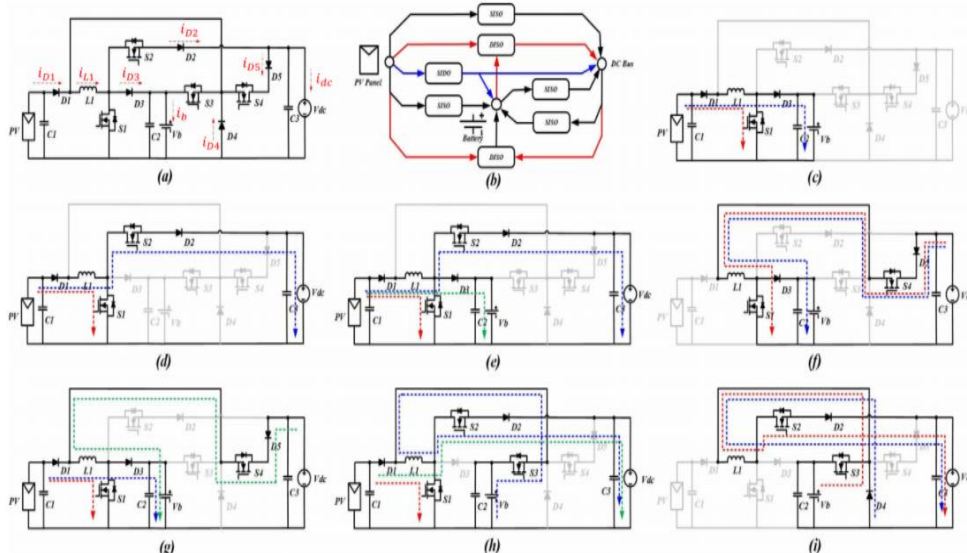
Fig. 2: Modes of Operation [11].
