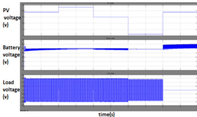
Fig. 10: Voltages of PV Panel, Battery and Load at Load on Condition.
