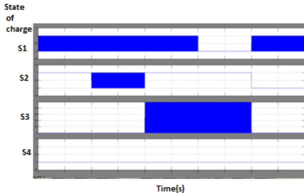
Fig. 9: Status of Switches S_1 , S_2 , S_3 , S_4 at Load on Condition.
