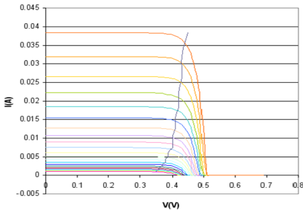
Fig. 5: Solar VI Curve in Varying Sunlight.
