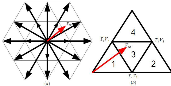
Fig. 6: Diagram Depicting Space Vector for (A) All Sectors (B) Sector 1.
