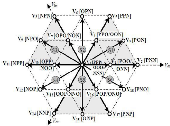
Fig. 5: Diagram Demonstrating Space Vector for A three (Three)-Level Inverter.
