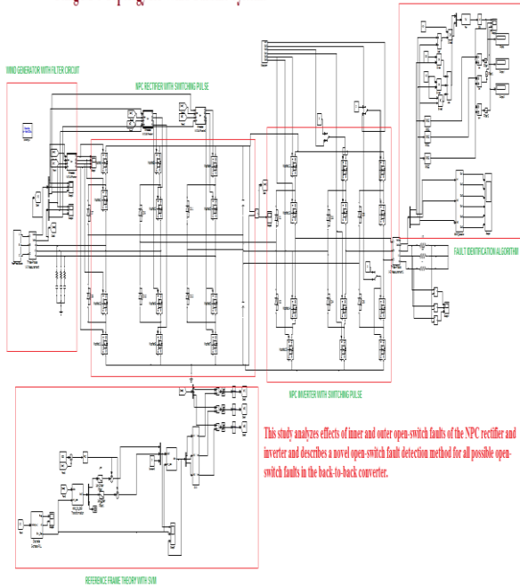
Fig. 9: Simulation Implementation of the Npc Back-To-Back Converter.
