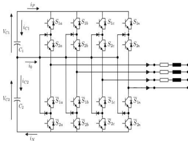
Fig. 4: A 3-Phase Neutral Point Clamped Inverter with 3-Levels.
