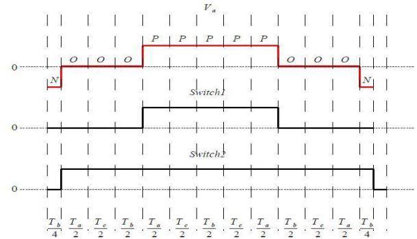
Fig. 7: Switching States Sequence Represented By Waveform For Switches 1 And 2 In Sector 1, Region 1, R-Phase.
