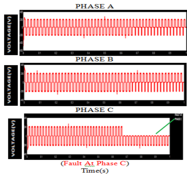
Fig. 12: Fault Occurrence In The Switch Open Switch Fault Occurs In The Switches.
