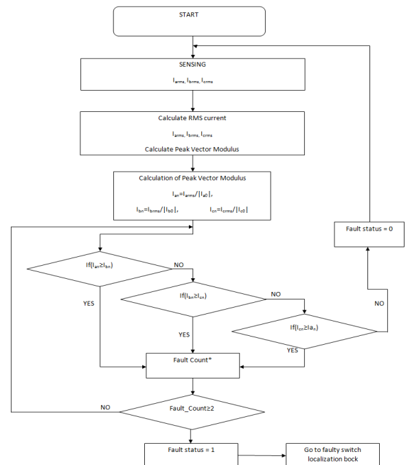
Fig. 8: Diagram Showing Open Switch Fault Detection Algorithm.
