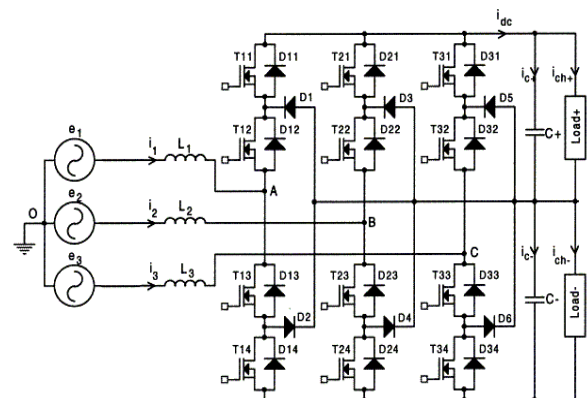
Fig. 2: Neutral Point Clamped Rectifier Including Three Levels.
