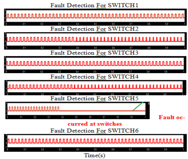
Fig. 11: Inverter Output at with Fault Condition.
