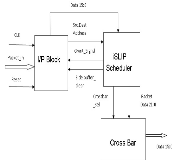
Fig .1: Single Node Noc Router.
