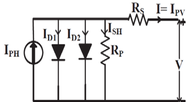
Fig. 3: Equivalent Circuit of PV Cell.
