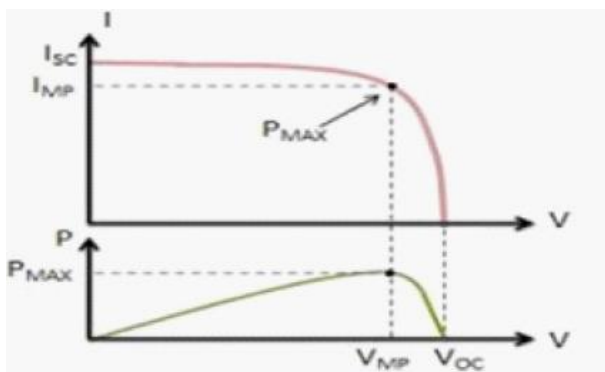
Fig. 5: Output Characteristics of PV Array.
