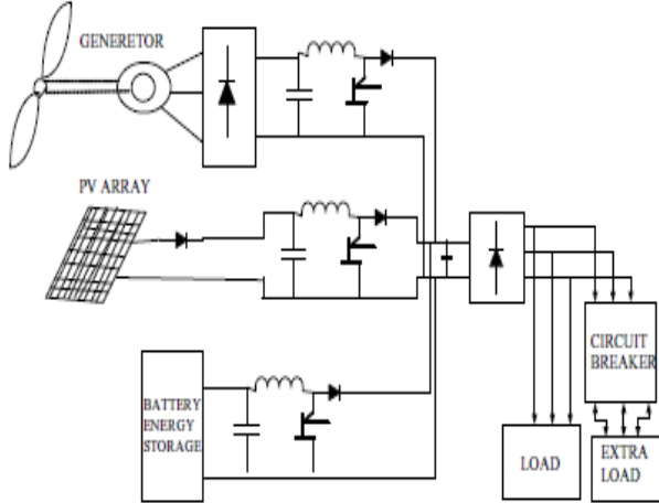
Fig. 1: Arrangement of Integrated Energy System.
