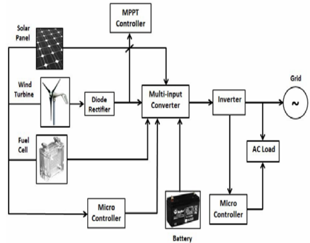
Fig. 2: Block Diagram of Hybrid System.
