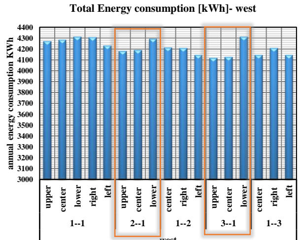
Fig9: the annual energy consumption in the different window position – in west –WWR 30%
