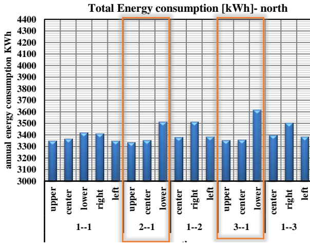
Fig 6: the annual energy consumption in the different window position – in north –WWR 30%
