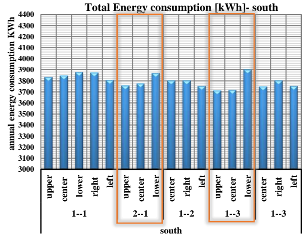
Fig 8: the annual energy consumption in the different window position – in south –WWR 30%
