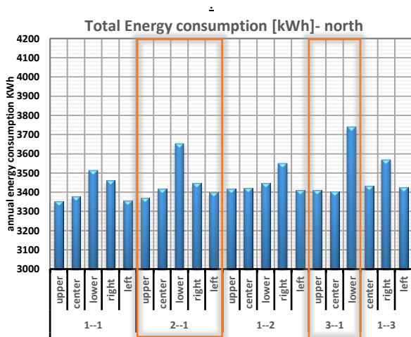
Fig 2: the annual energy consumption in the different window position – in north –WWR 20%
