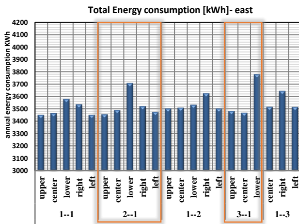
Fig 3: the annual energy consumption in the different window position – in east –WWR 20%
