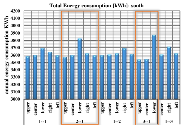
Fig4: the annual energy consumption in the different window position – in south –WWR 20%
