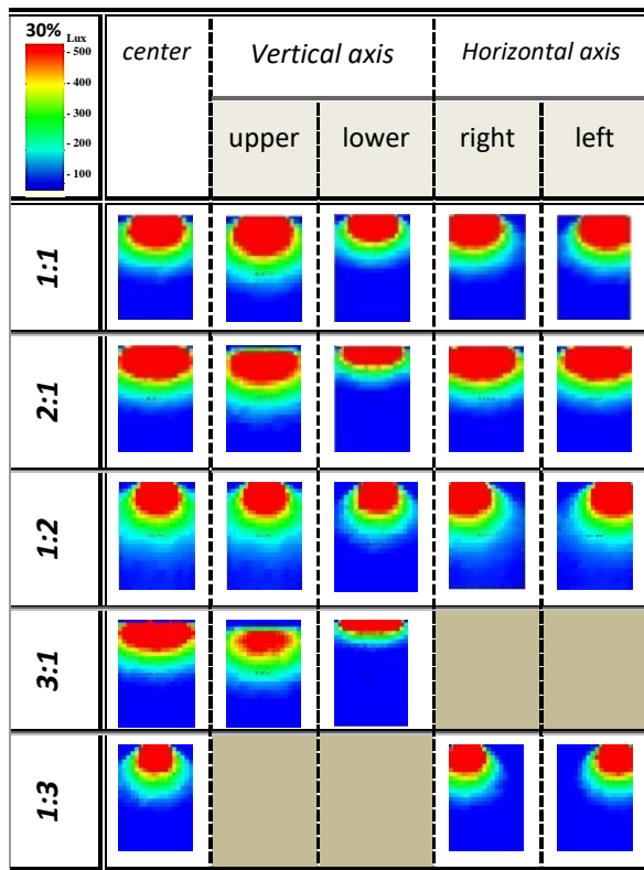
Fig 11: the distribution of light intensity in the different window position – in west–WWR 30%
