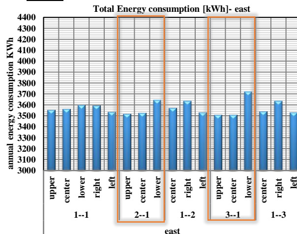
Fig7: the annual energy consumption in the different window position – in east –WWR 30%
