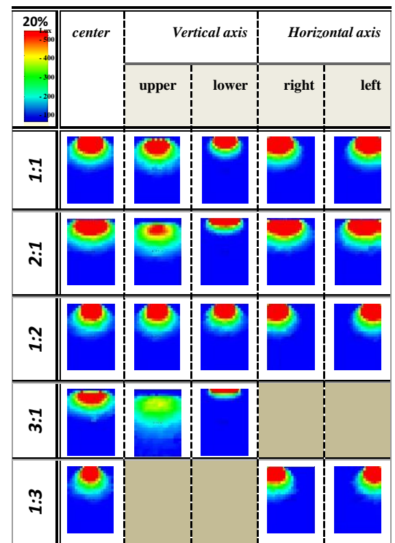
Fig10: the distribution of light intensity in the different window position – in west-WWR 20%
