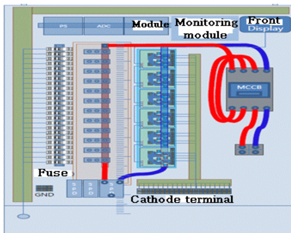
Fig. 2: Estimation of Device Installation in Connection Panel.
