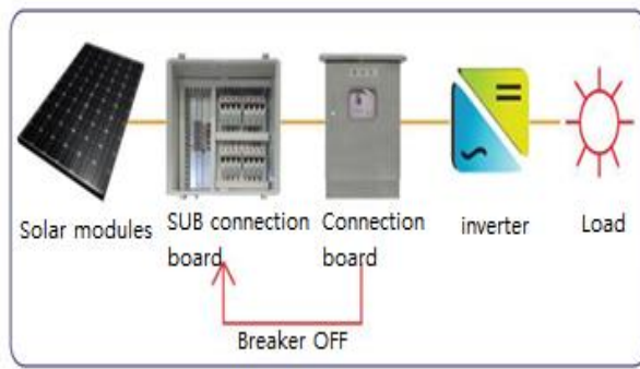
Fig. 1: Solar Monitoring System.
