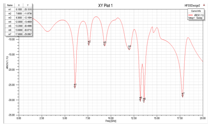
Fig. 2 Return loss
