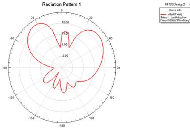
Fig. 3 Radiation Pattern
