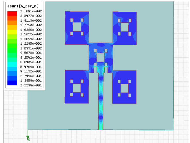
Fig. 5 Simulated Current Distributions
