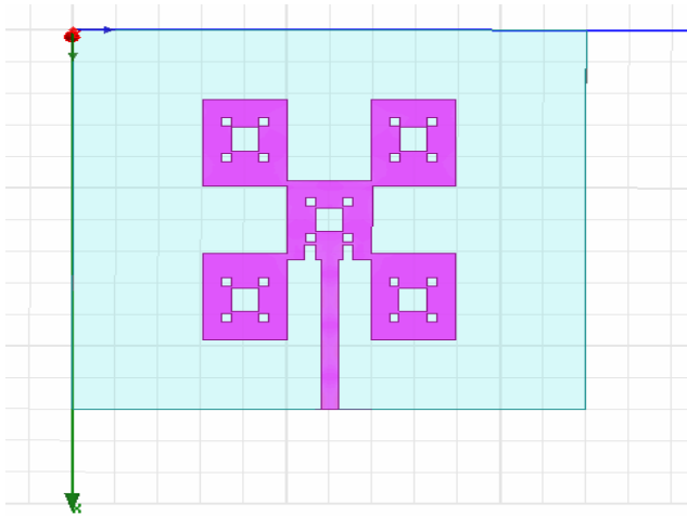
Fig.1 Geometry of the proposed antenna with top view
