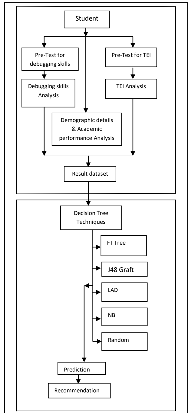
Fig. 1: Methodology Diagram.
