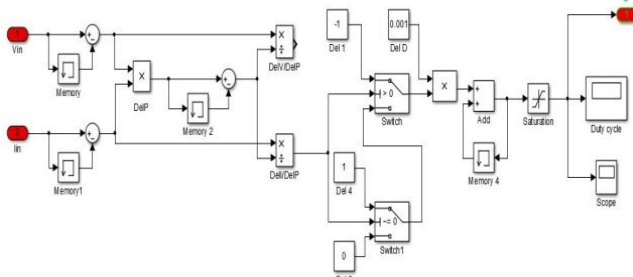
Figure 4: MPPT by using INC algorithm
