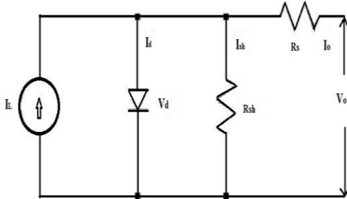
Figure 2: Single diode carved photovoltaic cell
