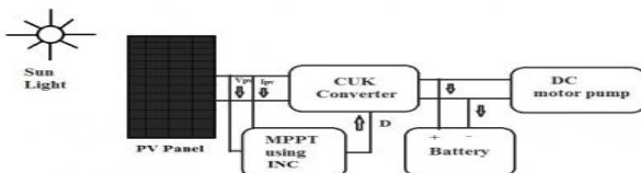
Figure 1: Basic block diagram of Proposed System
