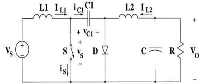
Figure 3: Circuit design for minimal Cuk converter
