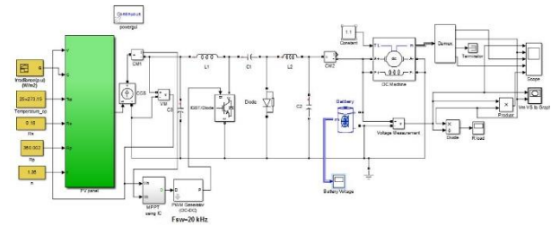
Figure 5: Overall Simulation diagram of proposed system
