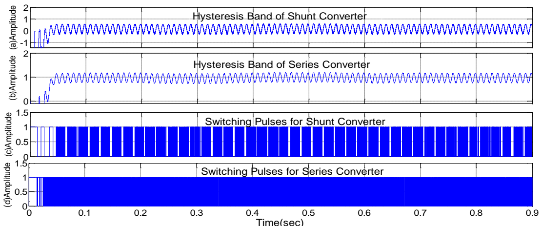
Fig. 13: Waveform of hysteresis band and Switching Pulses of Shunt and Series Inverter with AHBC.
