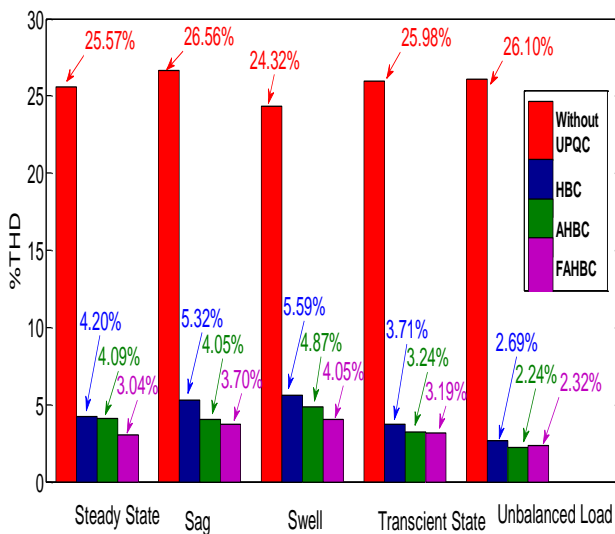
Fig. 20: Bar chart of Source Current Harmonics
