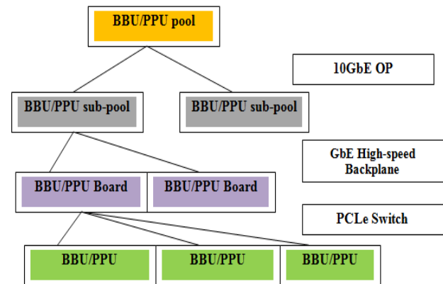
Fig. 2: Resource pooling framework in Evolved Node B
