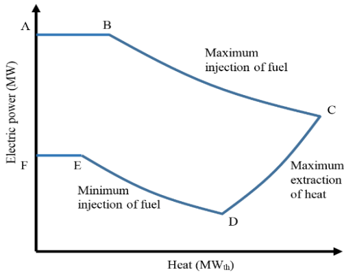
Fig. 1: CHP system feasible operation region.
