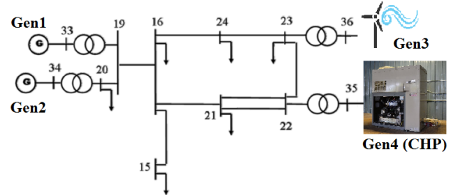
Fig. 5: A part of IEEE New England 39 bus power system
