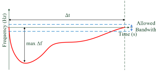
Fig. 2: Frequency behavior in load pick up of power system restoration
