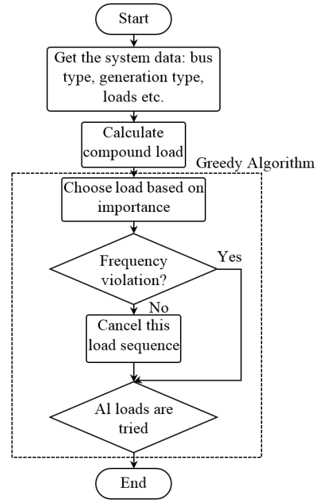
Fig. 4: Flowchart of proposed algorithm to power system restoration
