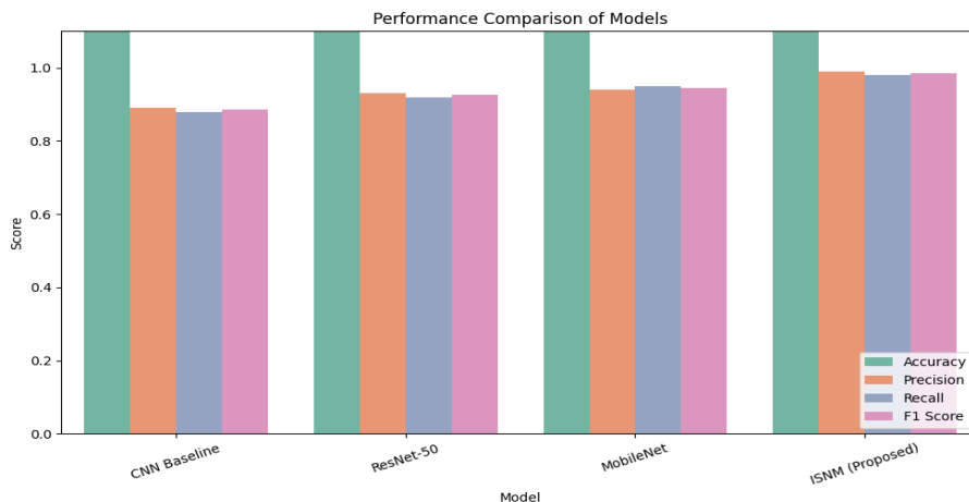
Fig. 4: Performance Analysis of Classifier.
