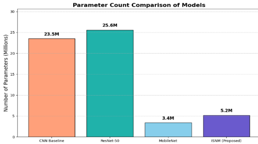
Fig. 3: Analysis of Parameter Count Comparison of Models.
