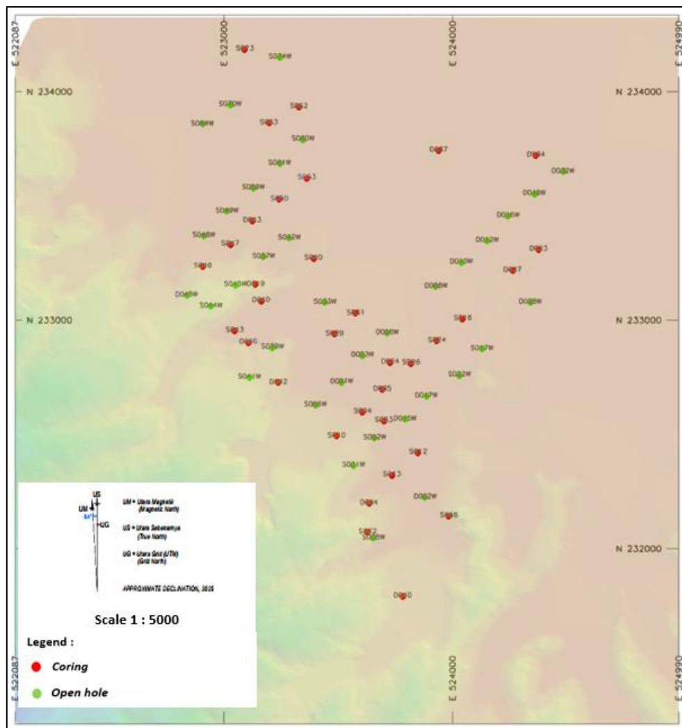
Fig 3: Distribution of drilling points at the Kelay Block 3 mine
