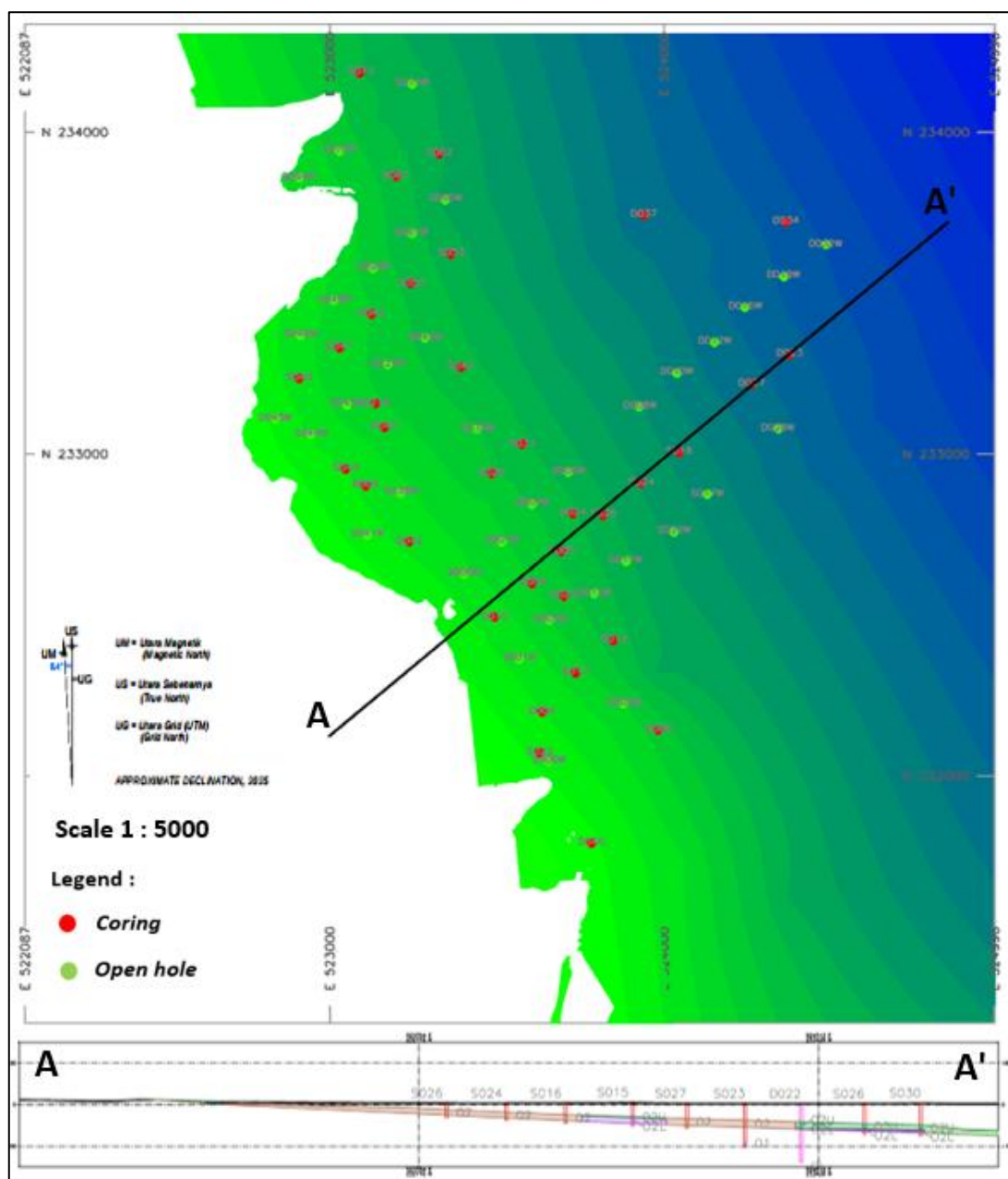
Fig 4: Geometric modeling and coal seam cross-section at the Kelay Block 3 area
