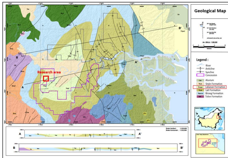
Fig 1: Regional geological map of the Tanjung Redeb sheet, East Kalimantan (Situmorang and Burhan, 1995).
