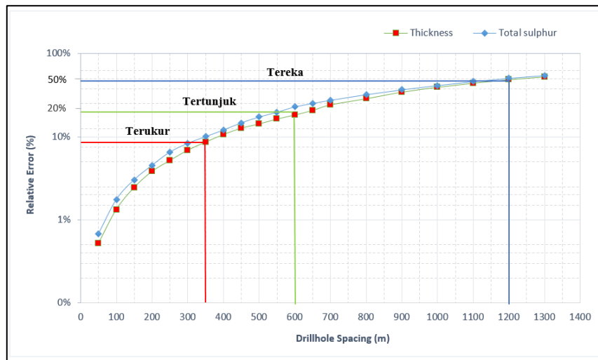
Fig 5 :Plot of relative error values with borehole scenario
