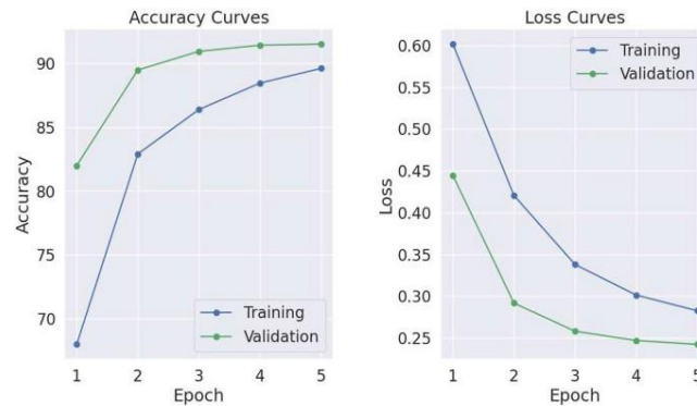
Fig. 3: Training and Validation Curves for Sentiment Models.
