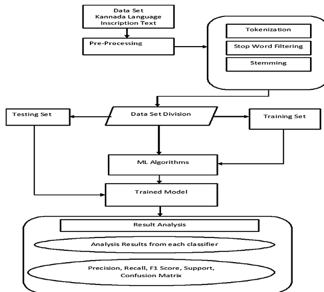
Fig. 3: Process flow execution diagram of the model.
