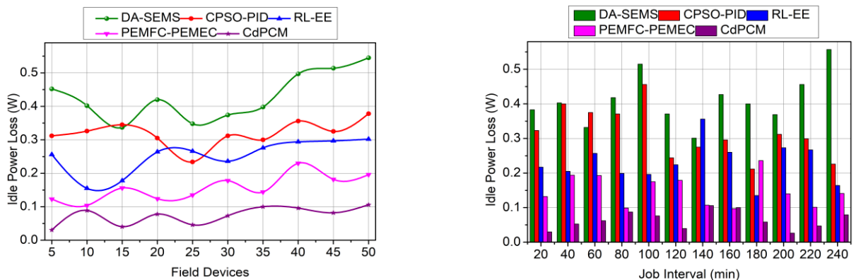
Fig. 9: Power Loss.
