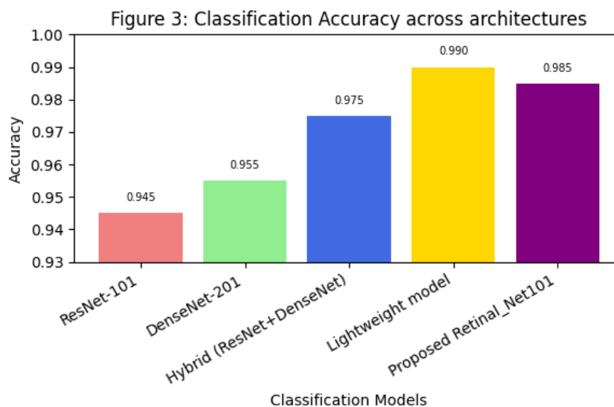
Fig. 3: Classification Accuracy across architectures
