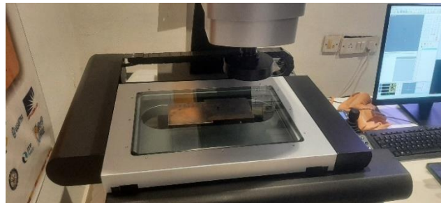
Fig. 3: Measuring kerf width of machined Nimonic alloy 75 sample by Video Profile Projector
