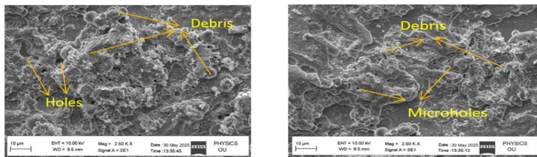
Fig. 9: Microstructure of Nimonic alloy 75 with non-treated and cryogenically treated brass wires
