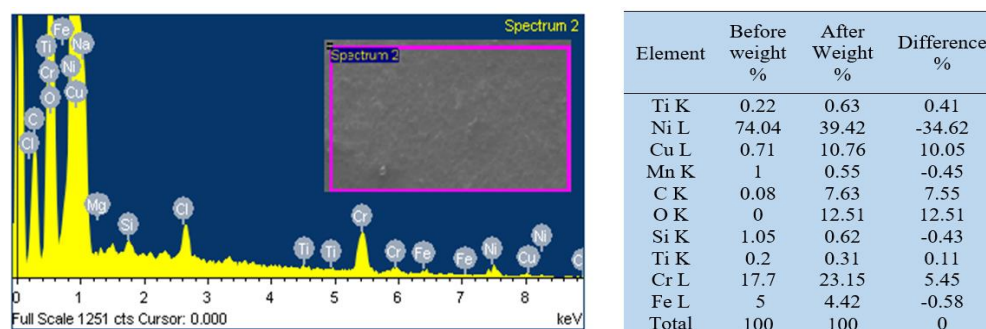
Fig. 11: EDS Result of sample No.6
