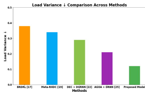
Fig. 12: Performance Metrics of Load Variance.
