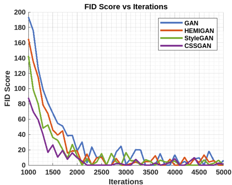
Fig. 8: FID Score vs. Iterations for CSSGAN and Other GAN Models
