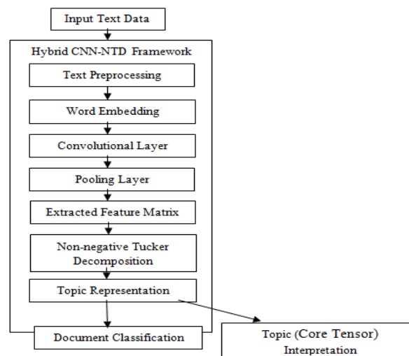
Fig. 2: Hybrid Convolutional Neural Networks with NTD (HCNN-NTD).
