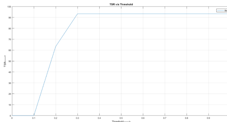
Fig. 11: TSR Verses Threshold Graph.
