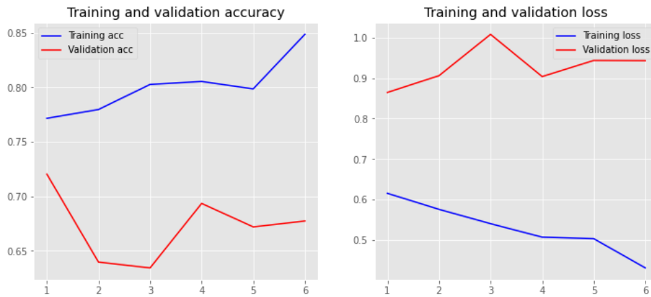
Fig.7: Bidirectional LSTM validation, training accuracy, and loss
