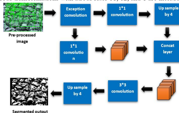
Fig. 6: DeepLabv3+Architecture.
