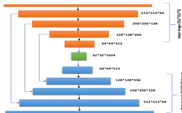
Fig. 5: UNET Architecture.
