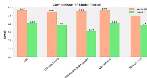
Fig. 4: KNN Recall.
