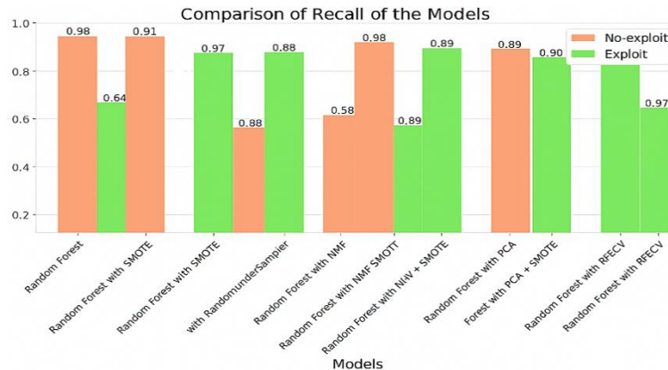
Fig. 7: Recall Comparison of Random Forest Models.
