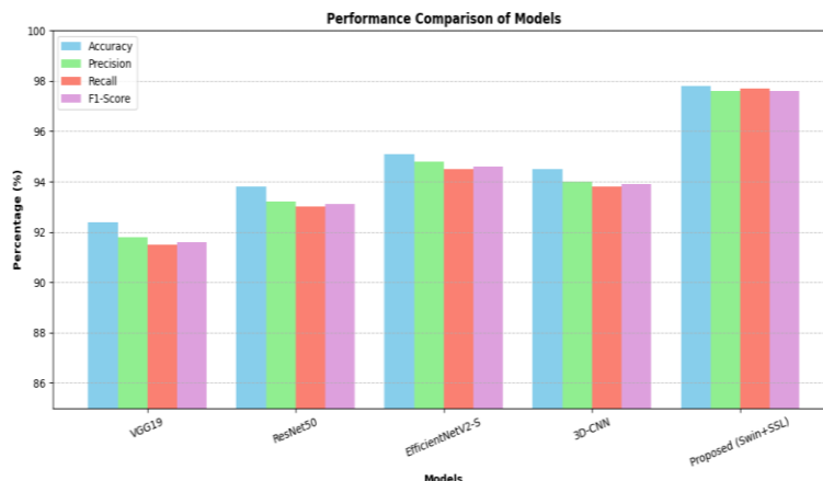
Fig. 6: Performance Comparison of All the Models.
