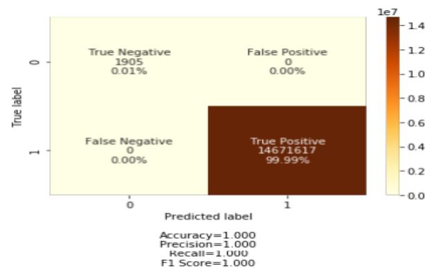
Fig. 7: Performance of the Proposed Model.
