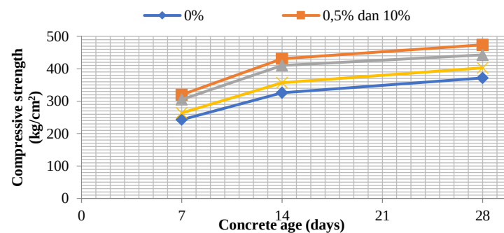
Fig. 6: Comparative Graph of the Compressive Strength of Normal Concrete and Concrete with the Addition of Superplasticizer and Iron Powder.
