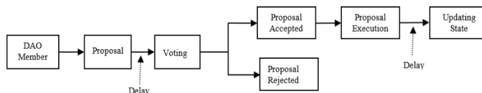
Fig. 3: On-Chain Governance Mechanism.
