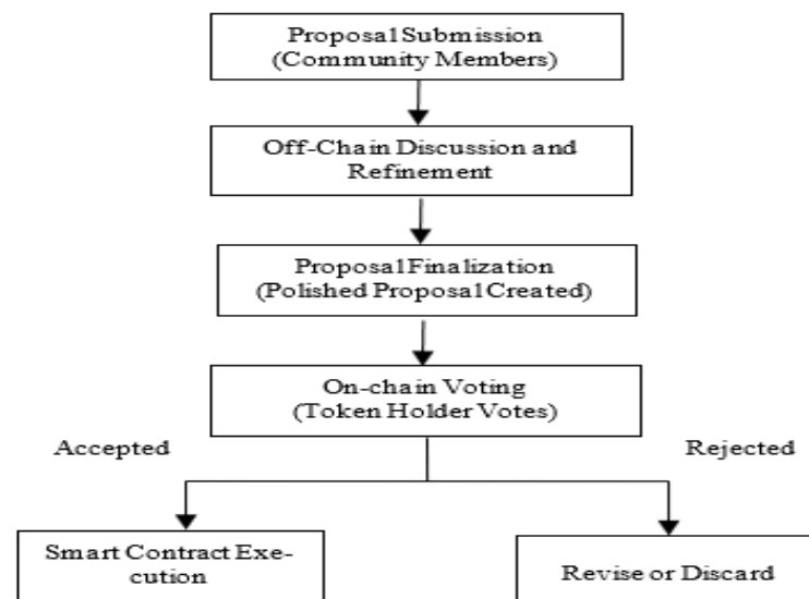
Fig. 4: Hybrid Governance Mechanism.
