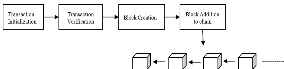
Fig. 1: Blockchain Transaction.
