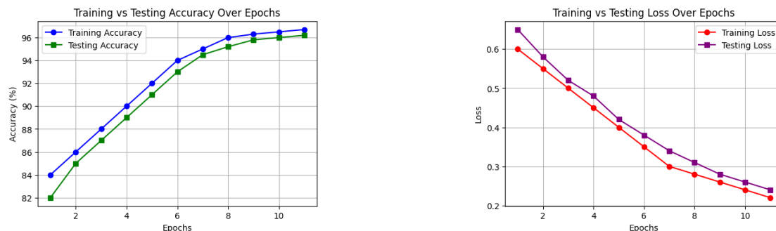
Fig. 11: Training vs Testing Accuracy and Loss.
