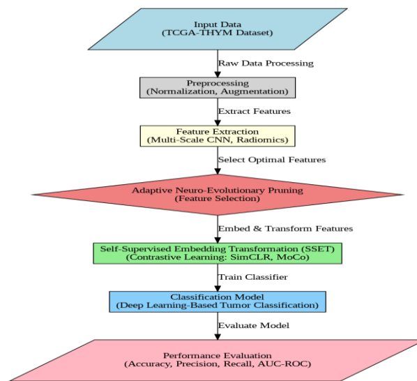
Fig. 2: Workflow of the proposed work.
