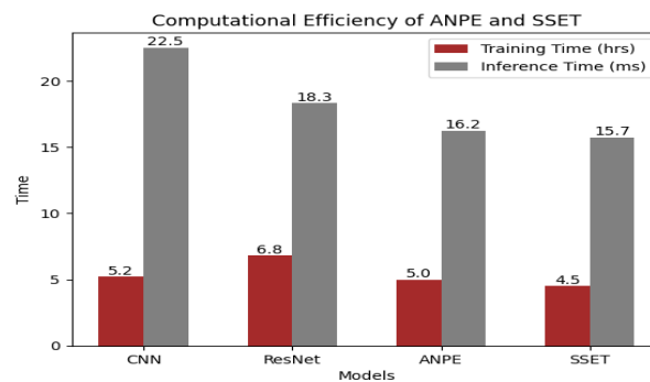
Fig. 9: Computational Efficiency Analysis.
