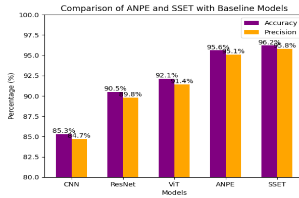
Fig. 6: Comparison of ANPE and SSET with Baseline Models.
