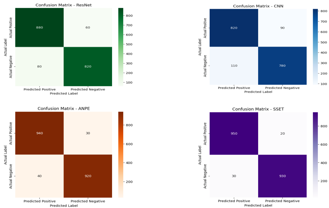
Fig. 8: Confusion Matrix for ResNet, CNN, ANPE, SSET.
