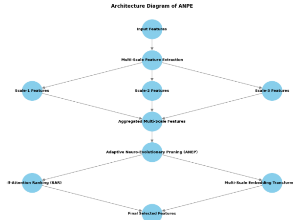
Fig. 4: Architecture Diagram of ANPE.
