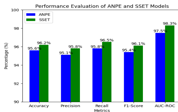
Fig. 5: Performance Metrics of ANPE and SSET Models.
