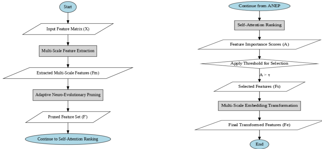
Fig. 3: Workflow of the Multi-Scale Feature Selection.
