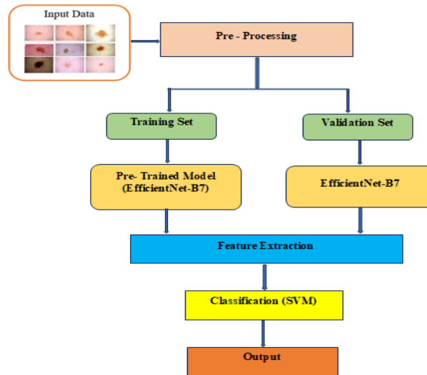
Fig. 1: Framework of Proposed Work
