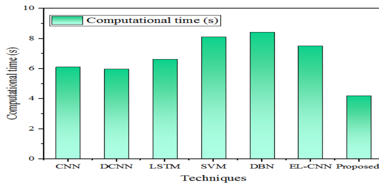
Fig. 12: Computational Time Comparison.
