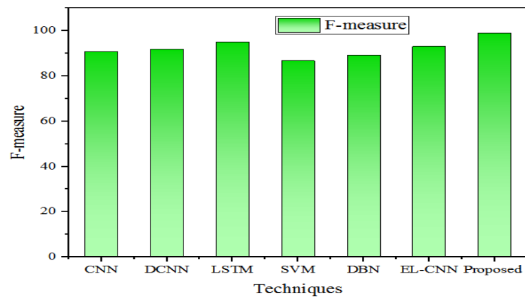
Fig. 10: F-Measure Comparison.
