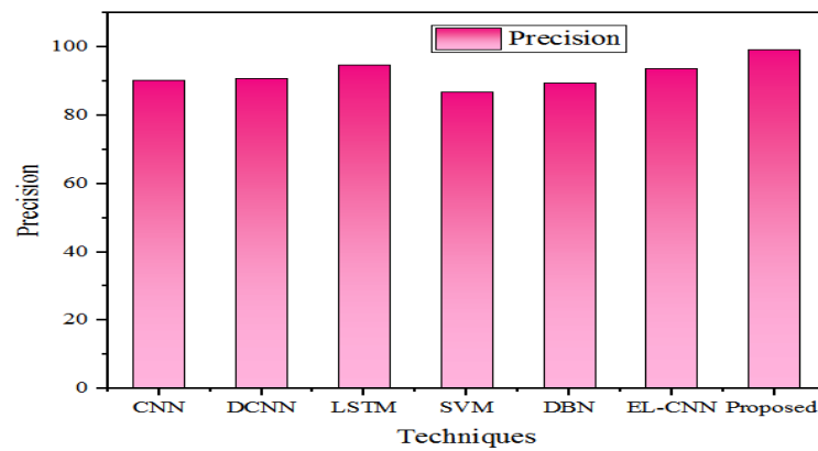
Fig. 8: Precision Comparison.
