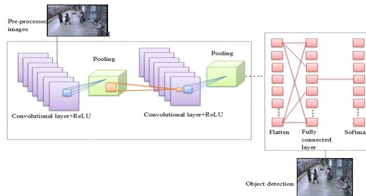
Fig. 3: CNN Architecture.
