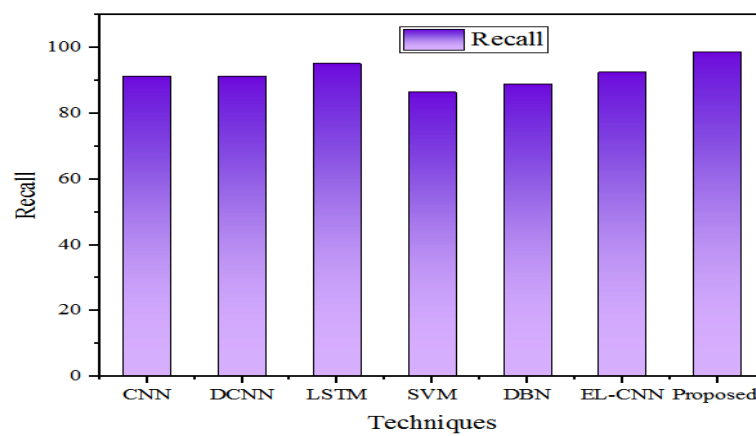
Fig. 9: Recall Comparison.
