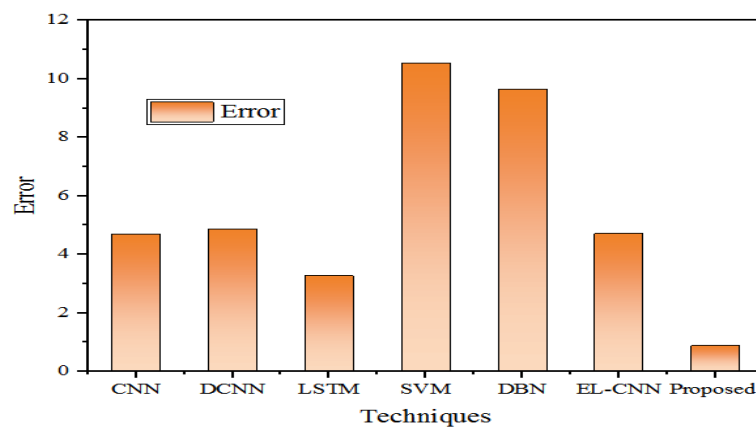
Fig. 11: Error Comparison.
