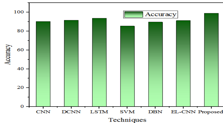
Fig. 7: Accuracy Comparison.
