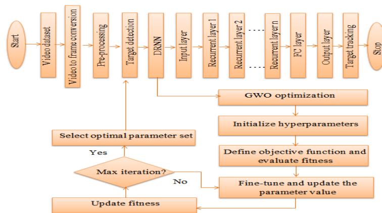
Fig. 4: Flowchart of the Developed Work.
