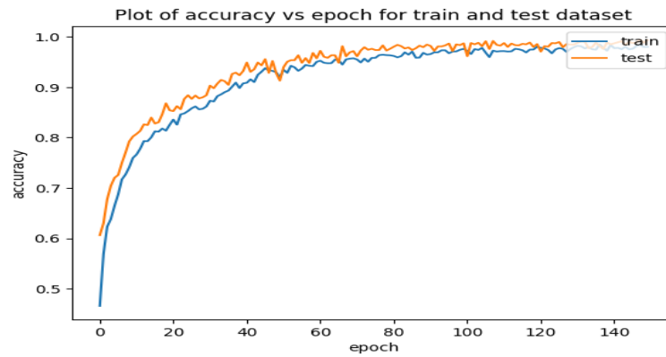
Fig. 5: Training and Testing Accuracy.
